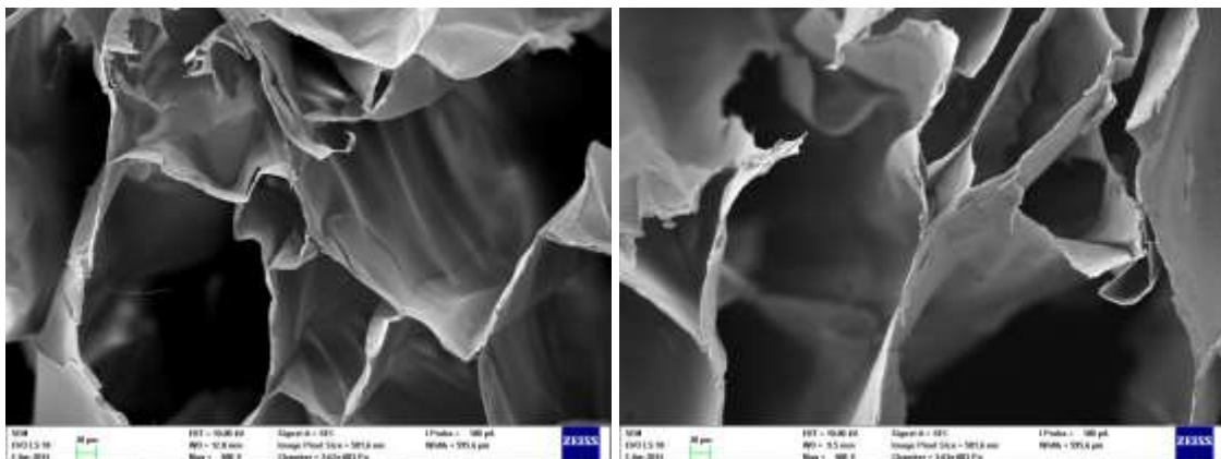
Fig. 3 Images for 1 wt. % agarose hydrogels (left) and for 1 wt. % agarose hydrogel with 1 wt. % lignohumate (right). A picture taken with 500-fold magnification and measure 20 µm.
