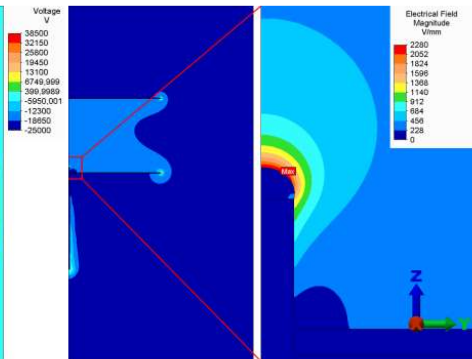
Fig. 5 Distribution of the electric field strength with a detailed view
