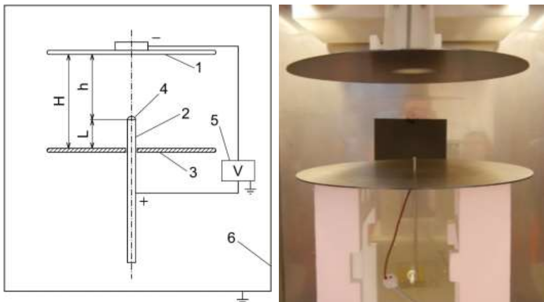
Fig. 1 Experimental apparatus
