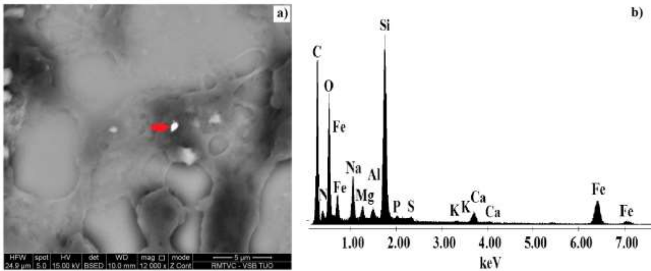
Fig. 3 SEM image of particle containing iron detected in the lung tumor tissue sample (a) with the corresponding EDX spectrum (b)
