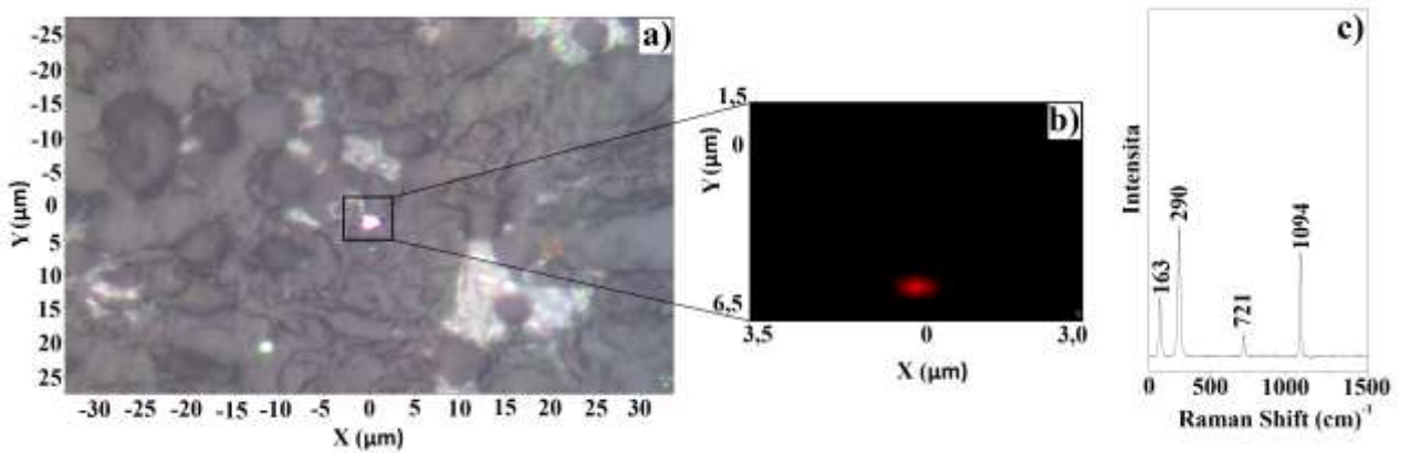
Fig. 1 Raman spectral map of the selected area of the lung cancer tissue, where a) light microscopy image of the tissue with the selected area, b) the spectral map of the selected area (red - siderite, black - surrounding tissue) and c) the measured Raman spectrum of siderite
