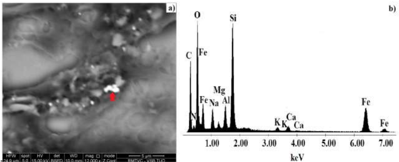
Fig. 4 SEM image of a cluster of particles containing iron detected in the lung tumor tissue sample (a) with the corresponding EDX spectrum (b)
