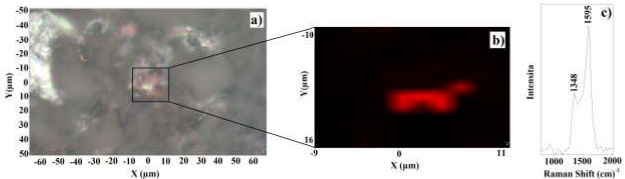
Fig. 2 Raman spectral map of the selected area of the lung cancer tissue, where a) light microscopy image of the tissue with the selected area, b) the spectral map of the selected area (red - carbon black, black - surrounding tissue) and c) the measured Raman spectrum of carbon black
