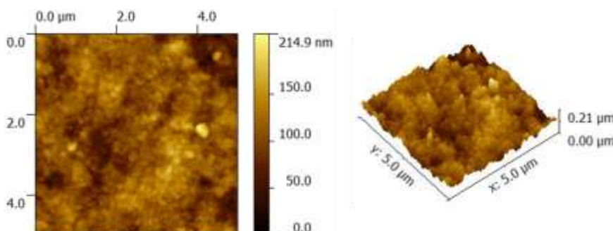
Fig. 3 AFM 2D and 3D images of PE2
