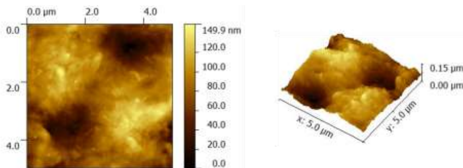
Fig. 5 AFM 2D and 3D images of PE/VerCA1
