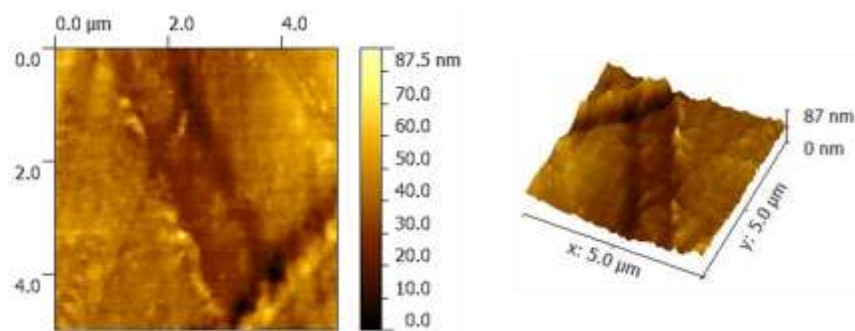
Fig. 4 AFM 2D and 3D images of PE/VerCA
