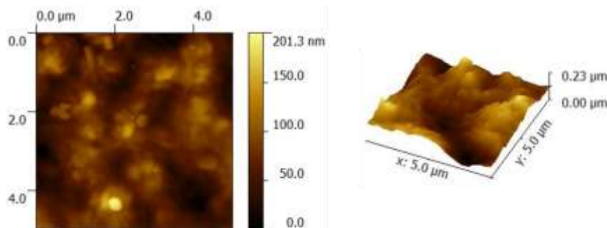
Fig. 2 AFM 2D and 3D images of PE1
