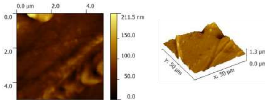
Fig. 1 AFM 2D and 3D images of pure polyethylene
