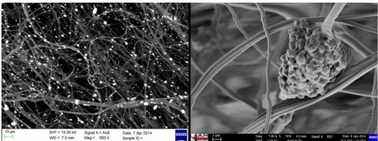
Fig. 1 Praseodymium tungstate particles in polymeric nanofibers, chemical (left) and topological (right) contrast
