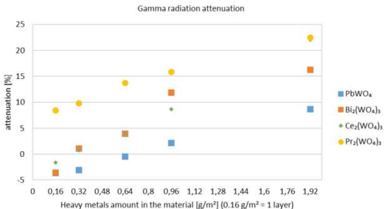
Fig. 2 Gamma radiation attenuation by a composite of polymer and heavy metal tungstates
