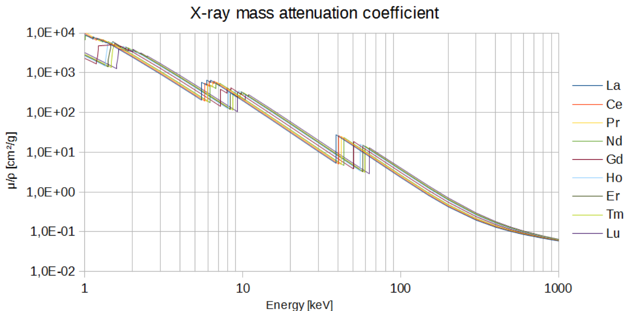
Fig. 3 X-Ray Mass attenuation coefficient (according to NIST; for elemental media)
