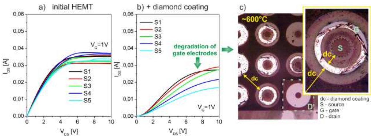
Fig. 1 Output characteristics of AlGaIn/GaN HEMTs without (a) and with (b) diamond coating (Note: labels S1-S5 correspond to different gate lengths; i.e. S1: L_g = 160 \mu\text{m} , S2: L_g = 140 \mu\text{m} , S3: L_g = 100 \mu\text{m} , S4: L_g = 60 \mu\text{m} , S5: L_g = 40 \mu\text{m} ). Fig. 1c) shows the top-view optical images of c-HEMTs after diamond deposition in focused MW plasma at different magnifications (the whole diameter of one circular-HEMT structure is 480 \mu\text{m} ).
