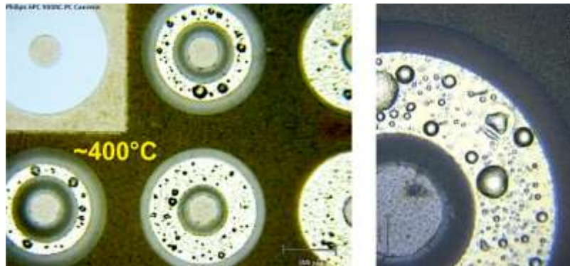
Fig. 2 Optical images of c-HEMTs after diamond deposition in linear antenna MW plasma at different magnifications (the whole diameter of one circular-HEMT structure is 480\ \mu\text{m} ).
